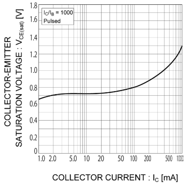
Fig.6 Collector emitter saturation voltage vs. collector current
