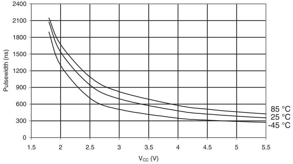
Figure 30-547. ATmega6450A: Minimum Reset Pulse Width vs. V_{CC}
