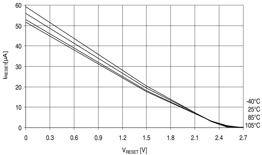
Figure 31-259. ATmega3250A: Reset Pull-up Resistor Current vs. Reset Pin Voltage ( V_{CC} = 2.7V )
