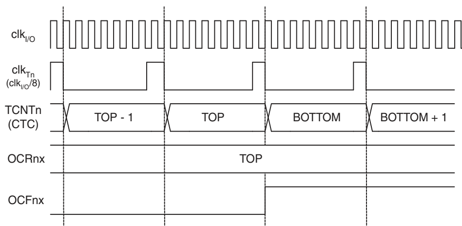
Figure 18-11. Timer/Counter Timing Diagram, Clear Timer on Compare mode, with Prescaler ( f_{clk\_I/O}/8 ).
