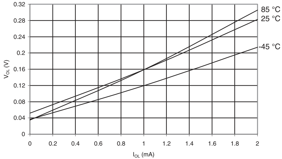
Figure 30-395. ATmega645A: I/O Pin Output Voltage vs. Sink Current, Ports A, C, D, E, F, G ( V_{CC} = 1.8V )
