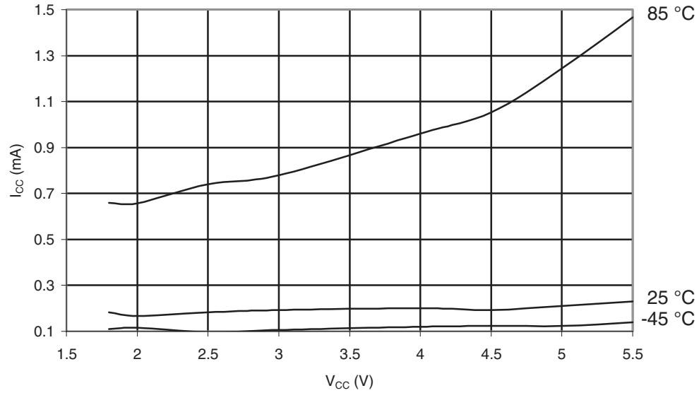
Figure 30-560. ATmega6450A: Power-down Supply Current vs. V_{CC} (32kHz Watch XTAL)
