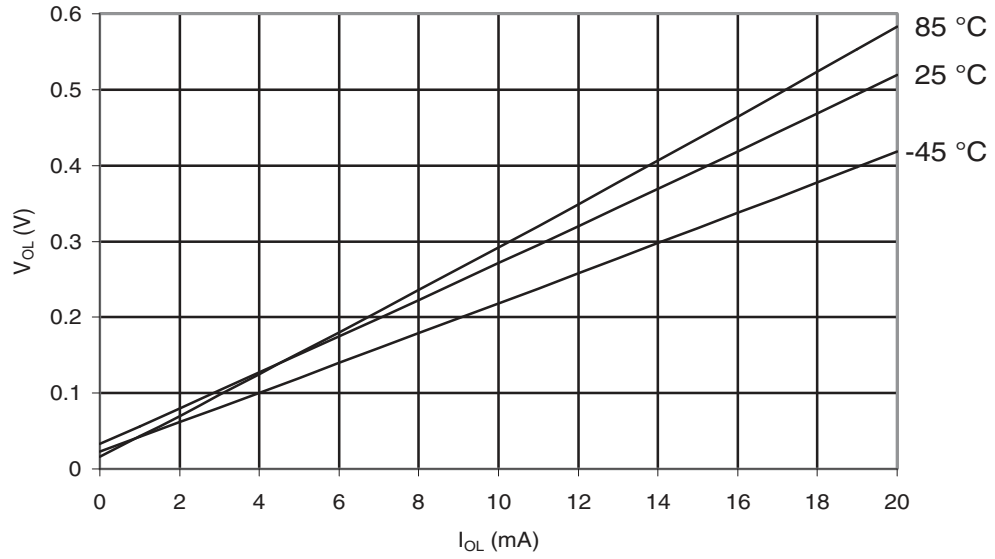
Figure 30-515. ATmega6450A: I/O Pin Output Voltage vs. Sink Current, Ports A, C, D, E, F, G, H ( V_{CC} = 5V )
