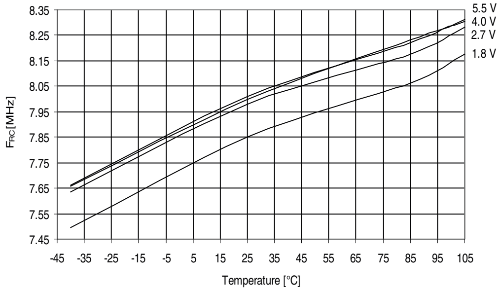
Figure 31-352. AATmega3250PA: Calibrated 8MHz RC Oscillator Frequency vs. Temperature
