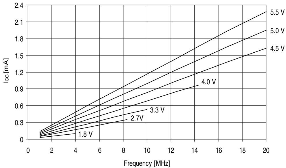
Figure 31-121. ATmega325A: Reset Supply Current vs. V_{CC} (1 - 20MHz, Excluding Current Through The Reset Pull-up)
