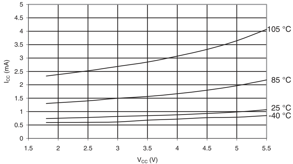
Figure 31-201.ATmega3250P: Standby Supply Current vs. V_{CC} (32kHz Watch Crystal, Watchdog Timer Disabled)
