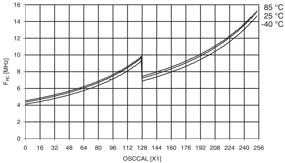
Figure 30-173. ATmega325A: Calibrated 8MHz RC Oscillator Frequency vs. OSCCAL Value
