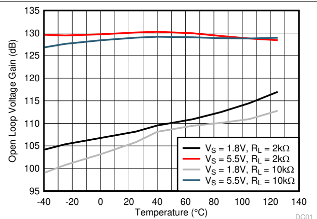
Figure 7-14. Open Loop Voltage Gain vs Temperature
