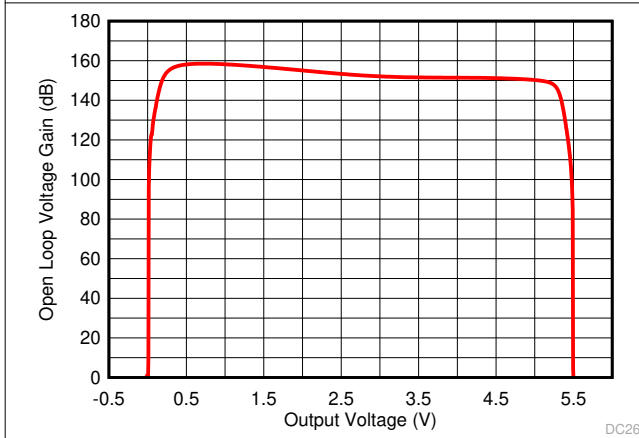
Figure 7-15. Open Loop Voltage Gain vs Output Voltage
