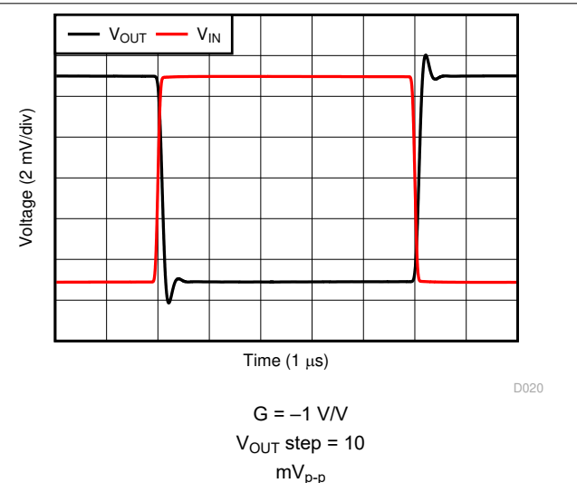
Figure 7-24. Small-Signal Step Response
