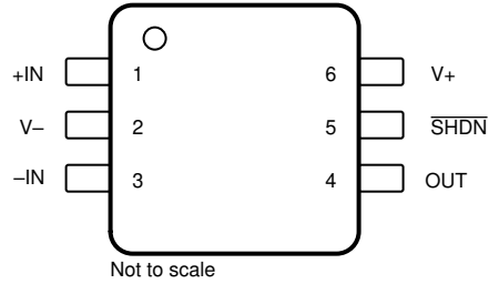
Figure 6-4. TLV9051S DBV Package 6-Pin SOT-23 Top View
