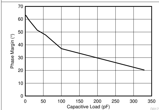
Figure 7-17. Phase Margin vs Capacitive Load
