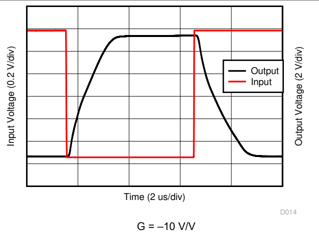
Figure 7-22. Overload Recovery
