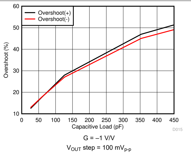
Figure 7-20. Small-Signal Overshoot vs Load Capacitance
