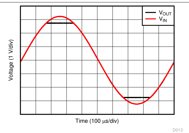
Figure 7-18. No Phase Reversal
