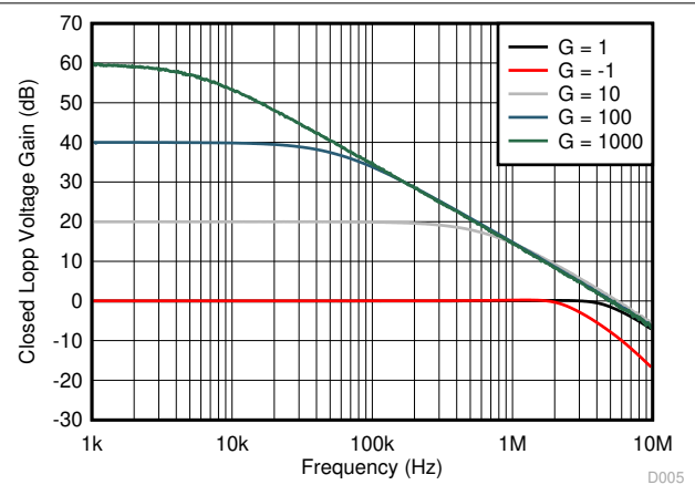
Figure 7-16. Closed Loop Voltage Gain vs Frequency
