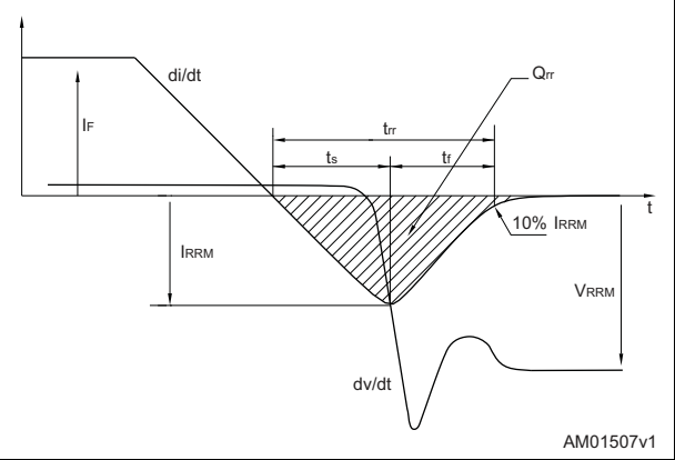
Figure 32. Diode recovery time waveform
