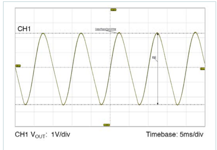
Figure 6 — Typical line frequency output voltage ripple waveform, T_{CASE} = 30^{\circ}C , V_{IN} = 230V , I_{OUT} = 6.9A , C_{OUT} = 6,800\mu F . Measured at C3, Figure 25
