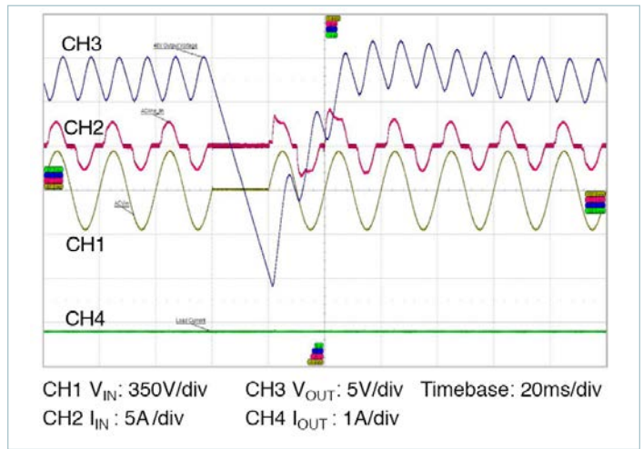
Figure 10 — Line drop out, 50Hz, 0^{\circ} phase, P_{LOAD} = 330W , C_{OUT} = 6,800\mu F
