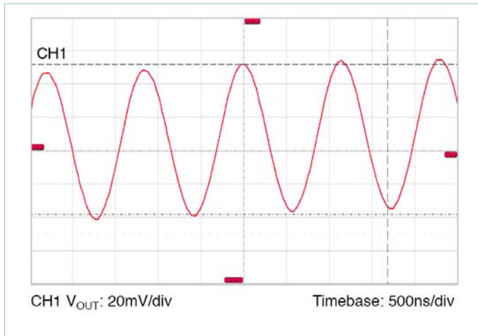
Figure 5 — Typical switching frequency output voltage ripple waveform, T_{CASE} = 30^{\circ}C , V_{IN} = 230V , I_{OUT} = 6.9A , no external ceramic capacitance
