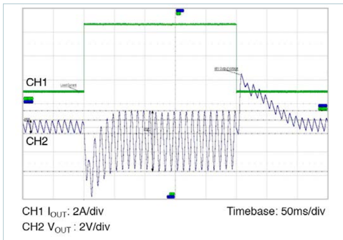
Figure 7 — Typical output voltage transient response, T_{CASE} = 30^{\circ}C , V_{IN} = 230V , I_{OUT} = 6.9A , C_{OUT} = 6,800\mu F
