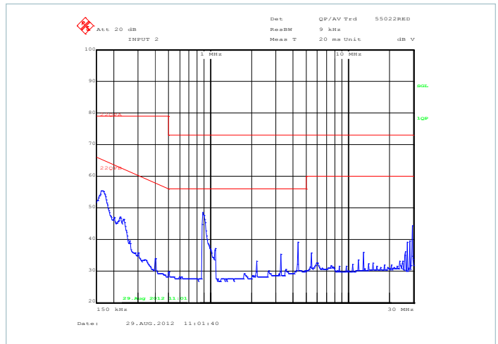
Figure 12 — Typical EMI spectrum, quasi-peak scan, 90% load, 230V_{IN} , C_{OUT} = 6,800\mu F ; test circuit – Figure 25
