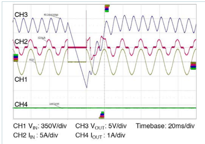
Figure 11 — Line drop out, 50Hz, 90^{\circ} phase, V_{IN} = 230V , P_{LOAD} = 330W , C_{OUT} = 6,800\mu F
