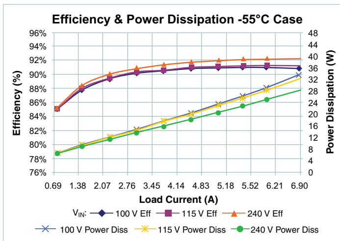
Figure 19 — V_{IN} to V_{OUT} efficiency and power dissipation vs. V_{IN} and I_{OUT} , T_{CASE} = -55^{\circ}C
