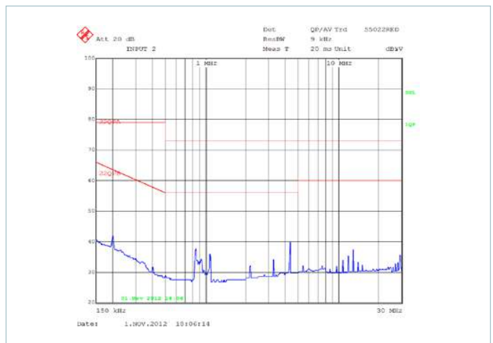
Figure 14 — Typical EMI spectrum, quasi-peak scan, 90% load, 115V_{IN} , C_{OUT} = 6,800\mu F ; test circuit – Figure 25
