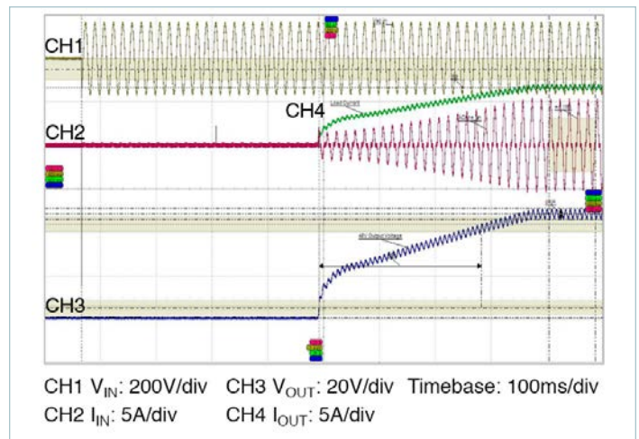
Figure 8 — Typical start-up waveform, application of V_{IN} , R_{LOAD} = 7.1\Omega , C_{OUT} = 6,800\mu F
