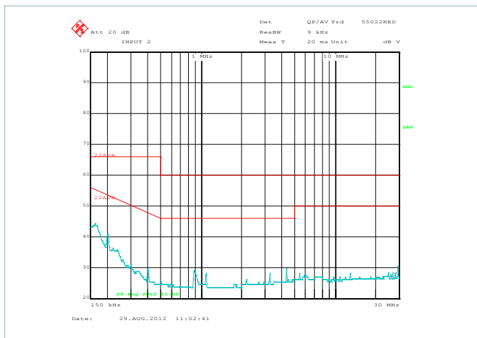
Figure 13 — Typical EMI spectrum, average scan, 90% load, 230V_{IN} , C_{OUT} = 6,800\mu F ; test circuit – Figure 28
