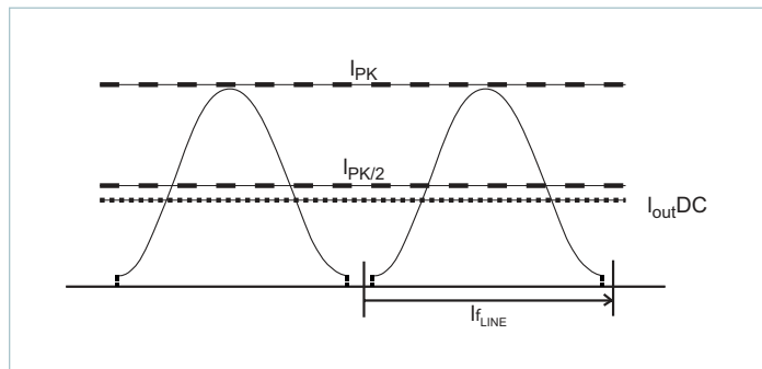
Figure 26 — Output current waveform
