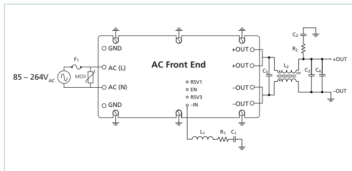
Figure 25 — Typical application for EN55022 Class B EMI
