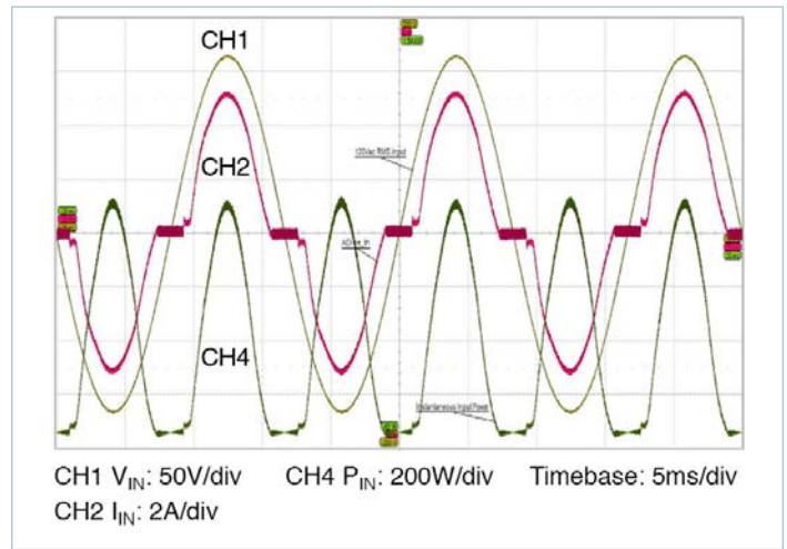
Figure 16 — Typical line current waveform, 60Hz, V_{IN} = 120V , P_{LOAD} = 330W ; C_{OUT} = 6,800\mu F
