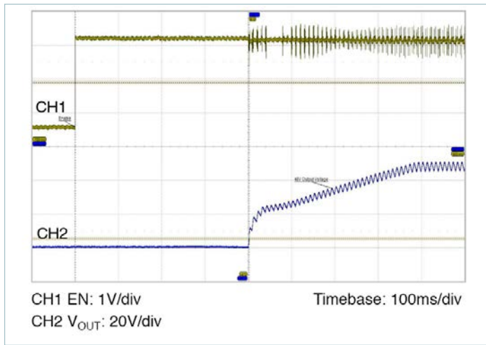
Figure 9 — Typical start-up waveform, EN pin release, V_{IN} = 230V , R_{LOAD} = 7.1\Omega , C_{OUT} = 6,800\mu F
