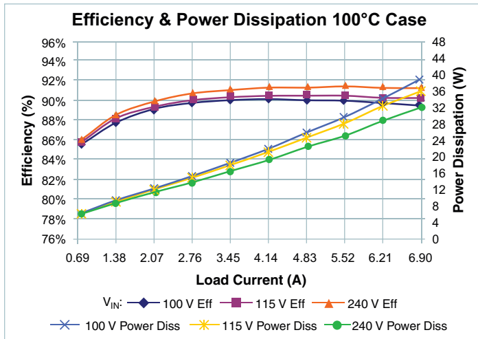
Figure 21 — V_{IN} to V_{OUT} efficiency and power dissipation vs. V_{IN} and I_{OUT} , T_{CASE} = 100^{\circ}C
