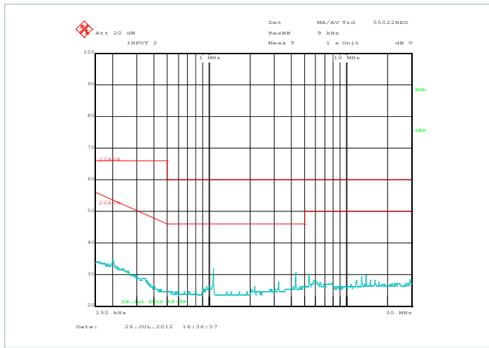
Figure 15 — Typical EMI spectrum, average scan, 90% load, 115V_{IN} , C_{OUT} = 6,800\mu F ; test circuit – Figure 25
