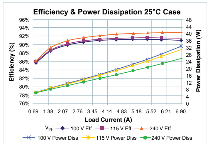
Figure 20 — V_{IN} to V_{OUT} efficiency and power dissipation vs. V_{IN} and I_{OUT} , T_{CASE} = 25^{\circ}C
