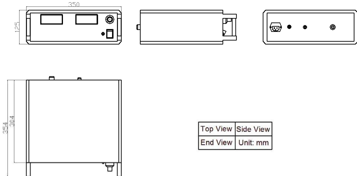
Figure 7. Dimensions for AHVACN60KVR5MABT
