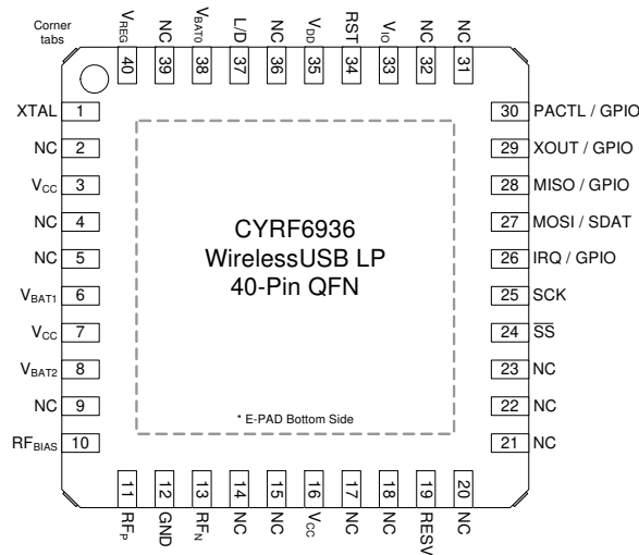
Figure 1. Pin Diagram - CYRF6936 40 QFN
