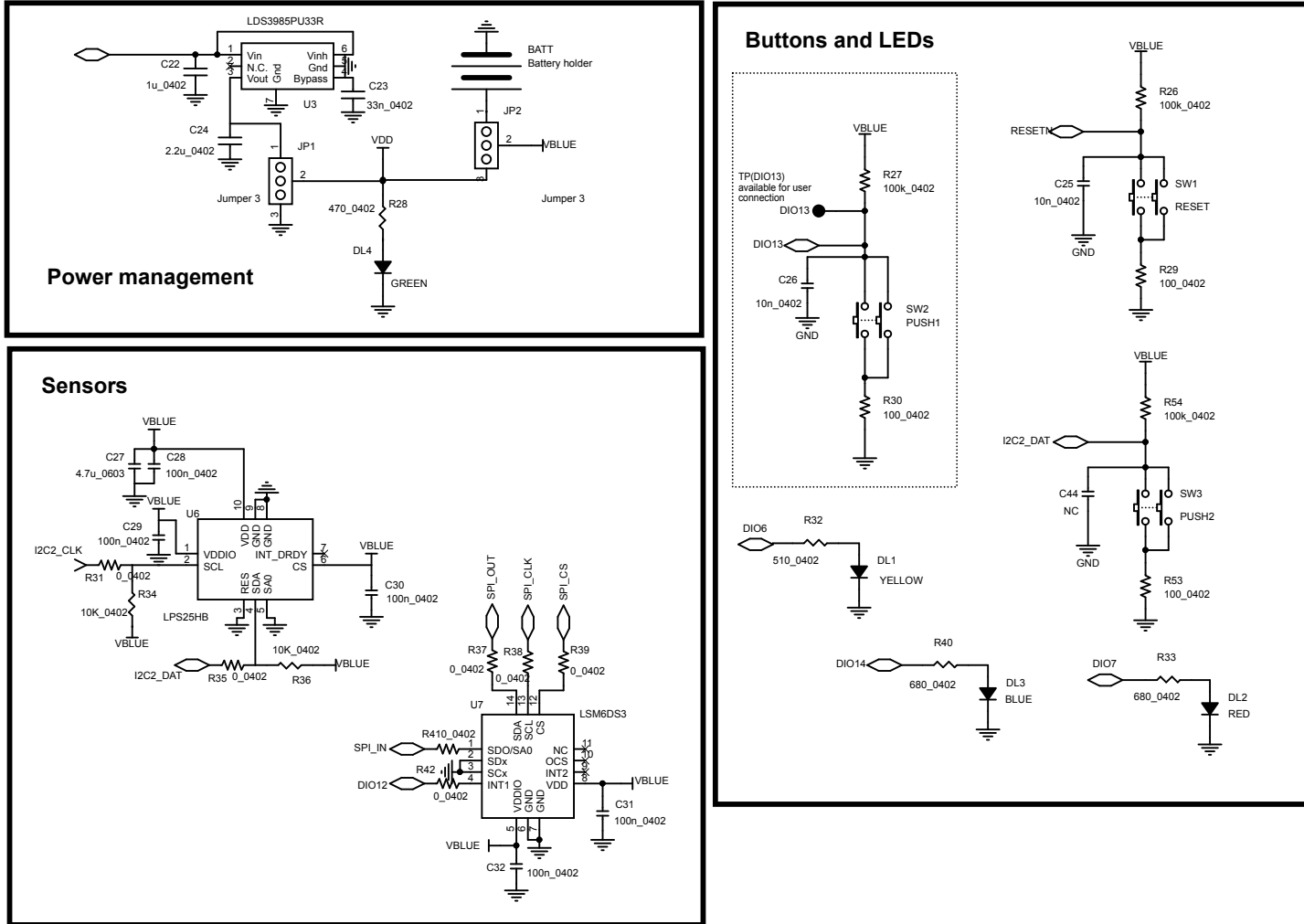
Figure 2. STEVAL-IBD008V1M circuit schematic (2 of 3)
