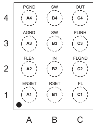
CSP-12 (Top View)
