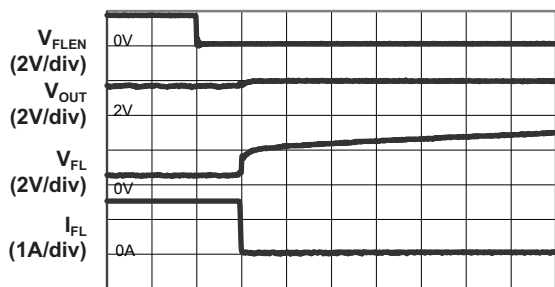
Flash Turn Off Characteristic
