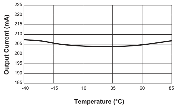
Movie Mode LED Current vs. Temperature ( I_{FL} = 206mA/Ch ; V_{IN} = 3.6V ; L = 1\mu H )
