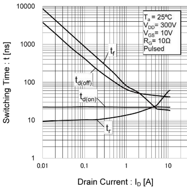
Fig.14 Switching Characteristics
