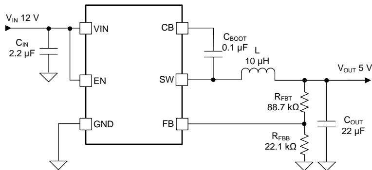
Figure 15. Application Circuit
