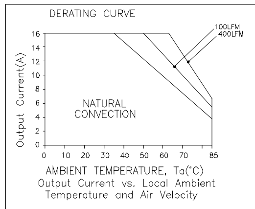
Figure 35. V_o = 5.0 V
