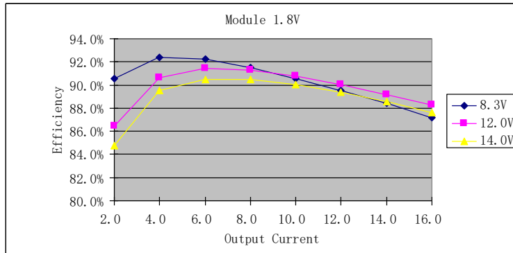
Figure 4. V_o = 1.8 V
