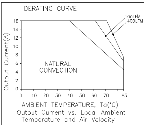
Figure 34. V_o = 3.3 V
