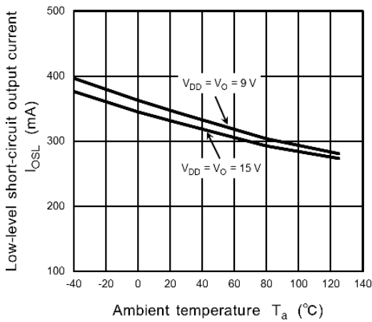
Fig. 12.2.9 I_{OL} - T_a
