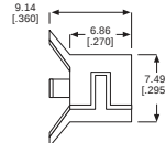
SPEED CLIP 515-0051
