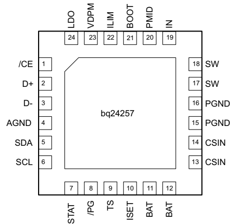
30-Pin DSBGA, 24-Pin QFN YFF, RGE Package (Top View)
