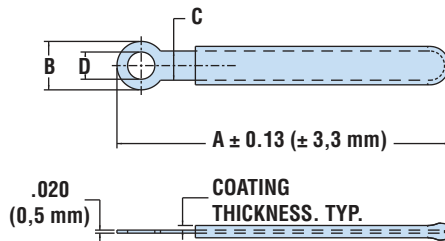
VCSC SCREW MOUNT
