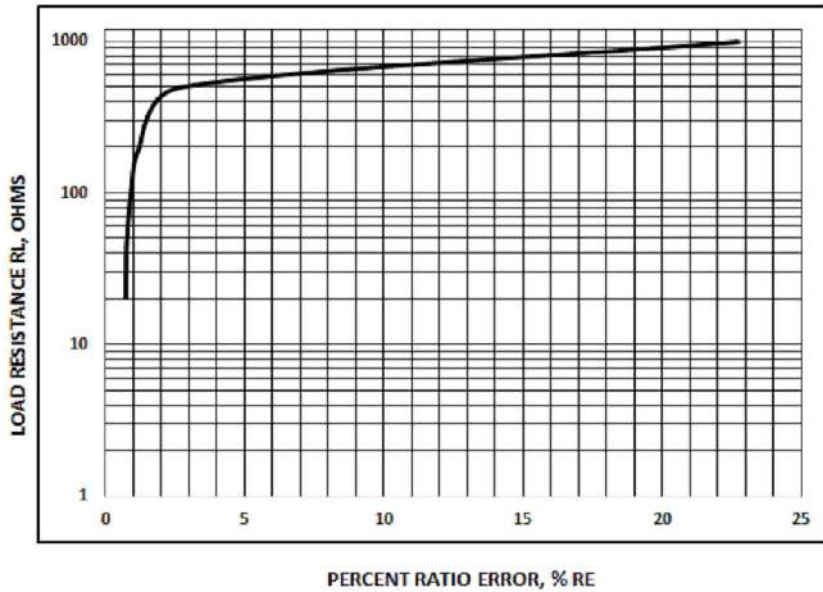
%RE VS RL AT RATED PRIMARY CURRENT @50A/50HZ
