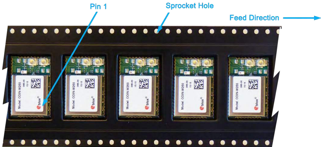
Figure 8: Orientation for ODIN-W2 modules on tape
