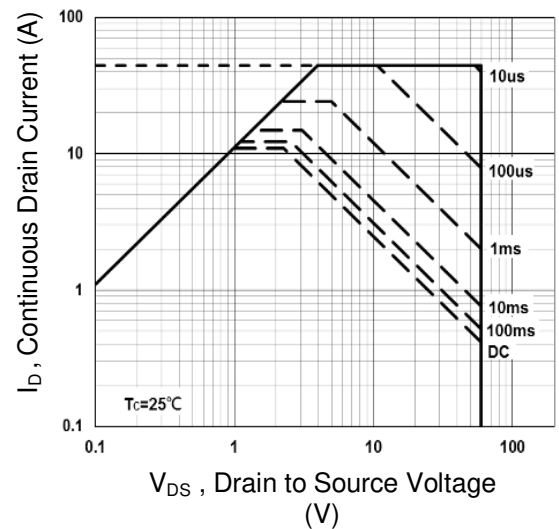
Maximum Safe Operation Area (TO-251S)
