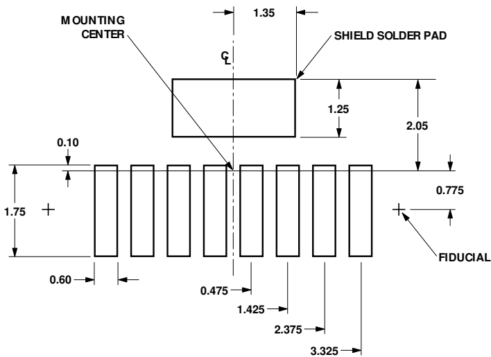
Figure 9. Land pattern.
