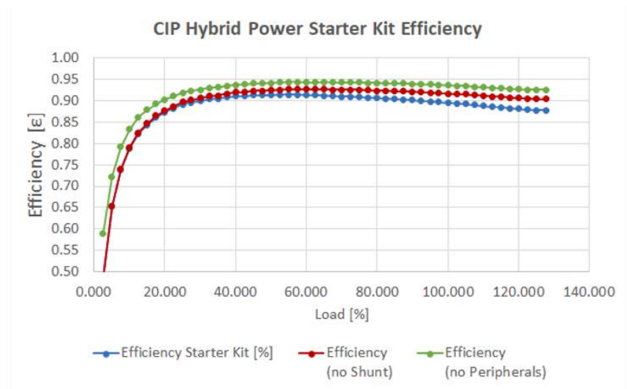
Figure 7-12. Efficiency Measurements
