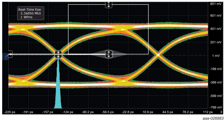
Fig. 5. HDMI 2.0 TP1 eye diagram, PCB with PHDMI2FR4 (2160p, 60 Hz)
