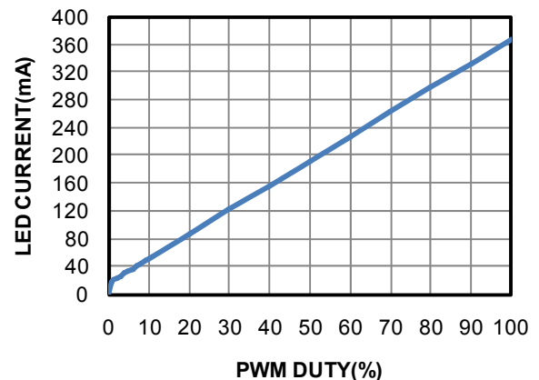
Dimming Curve
