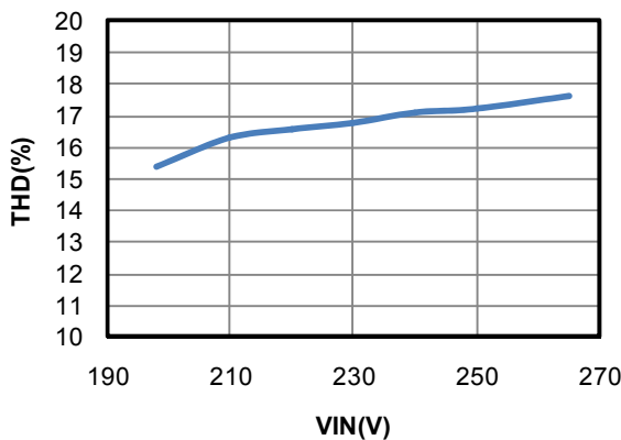
THD
