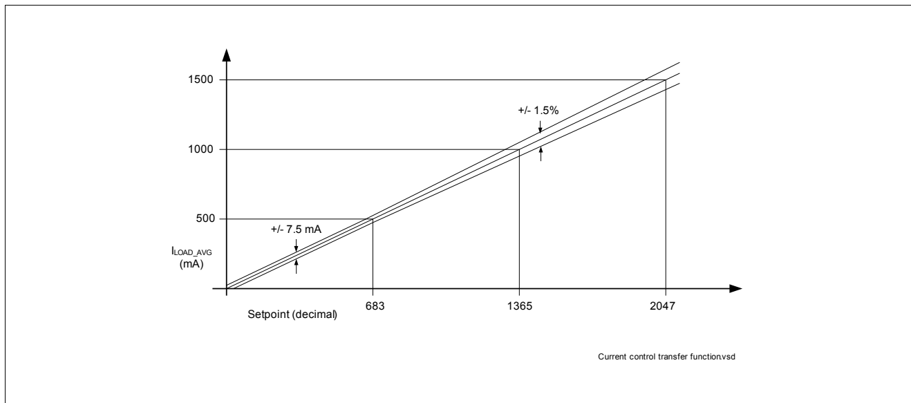
Figure 8 Output current transfer function and accuracy
