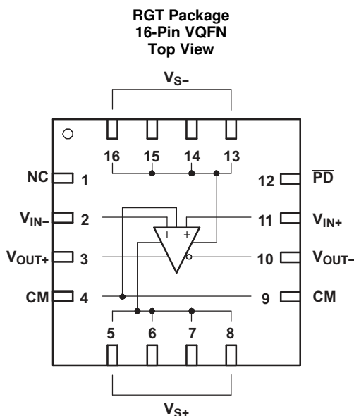
Pin Functions
