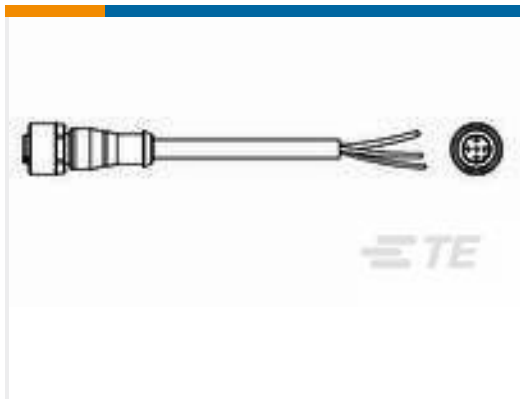
TE Part #2273029-3 M12 x 1.0 straight socket pigt A
