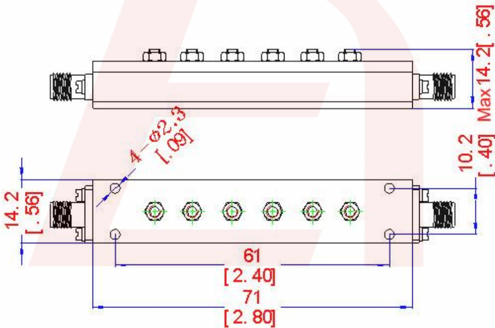
Outline Drawing:
