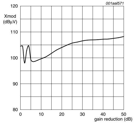
V_{DS(B)} = 5 V; V_{GG} = 5 V; V_{DS(A)} = V_{G1-S(A)} = 0 V; R_{G1} = 39 k \Omega (connected to V_{GG} ); f_w = 50 MHz; f_{unw} = 60 MHz; T_{amb} = 25 °C; see Figure 33 .
