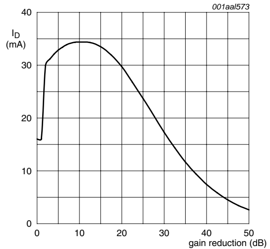
V_{DS(B)} = 5 V; V_{GG} = 5 V; V_{DS(A)} = V_{G1-S(A)} = 0 V; R_{G1} = 39 k \Omega (connected to V_{GG} ); f = 50 MHz; T_{amb} = 25 °C; see Figure 33 .
