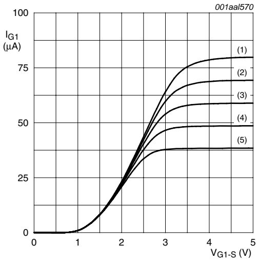
(1) V_{GG} = 5.0 V. (2) V_{GG} = 4.5 V. (3) V_{GG} = 4.0 V. (4) V_{GG} = 3.5 V. (5) V_{GG} = 3.0 V. V_{DS(B)} = 5 V; V_{DS(A)} = V_{G1-S(A)} = 0 V; T_j = 25 °C; R_{G1} = 39 k \Omega (connected to V_{GG} ); see Figure 2 .
