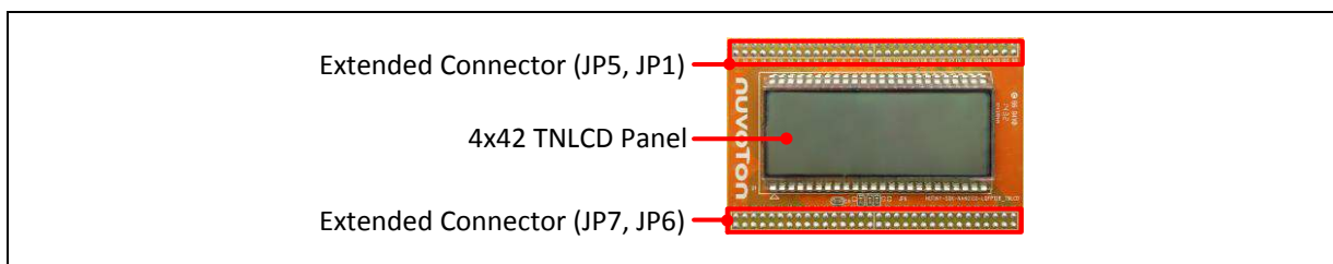
Figure 2-2 NuTiny-SDK-NANO130_TNLCD (PCB Board)
