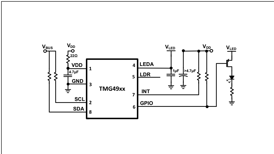
Figure 82: TMG4903 Typical Application Circuit
