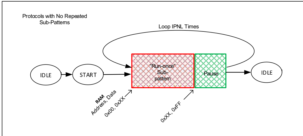
Figure 90: Complete Pattern Loops
