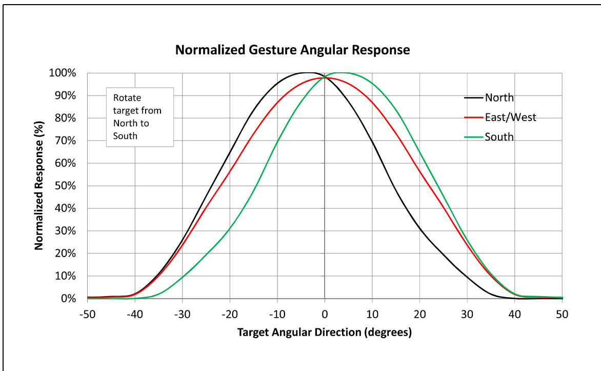
Figure 23: Gesture Angle Response
