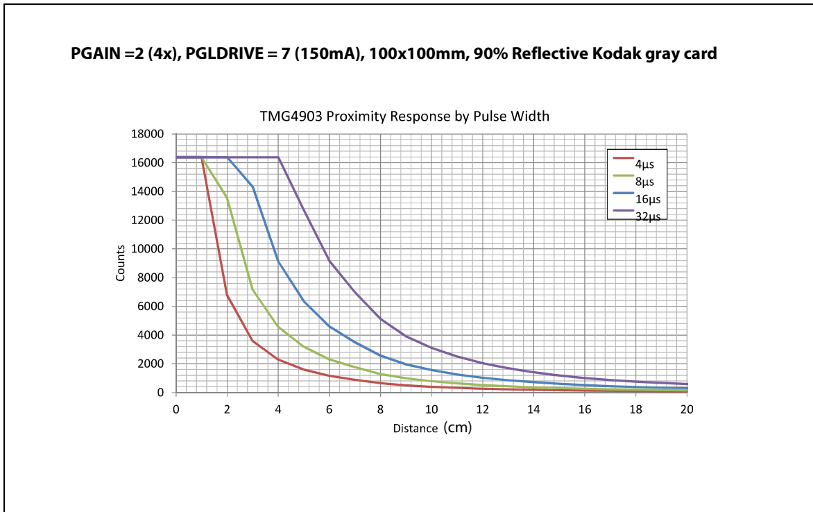
Figure 22: Gesture and Proximity Response vs. Target Distance
