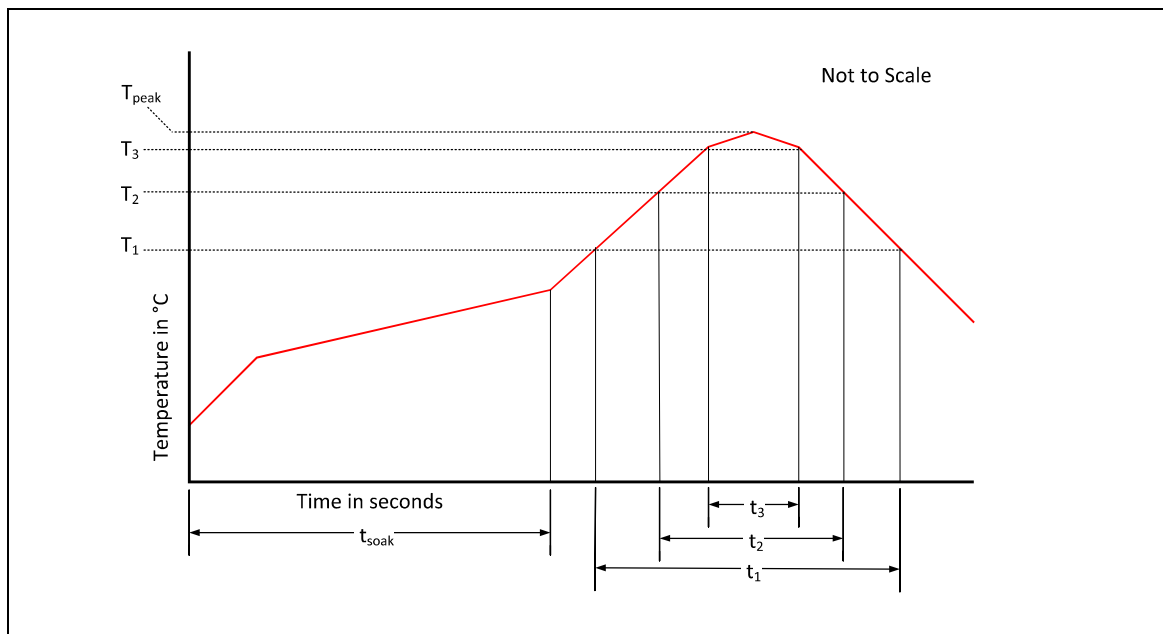
Figure 103: Solder Reflow Profile Graph
