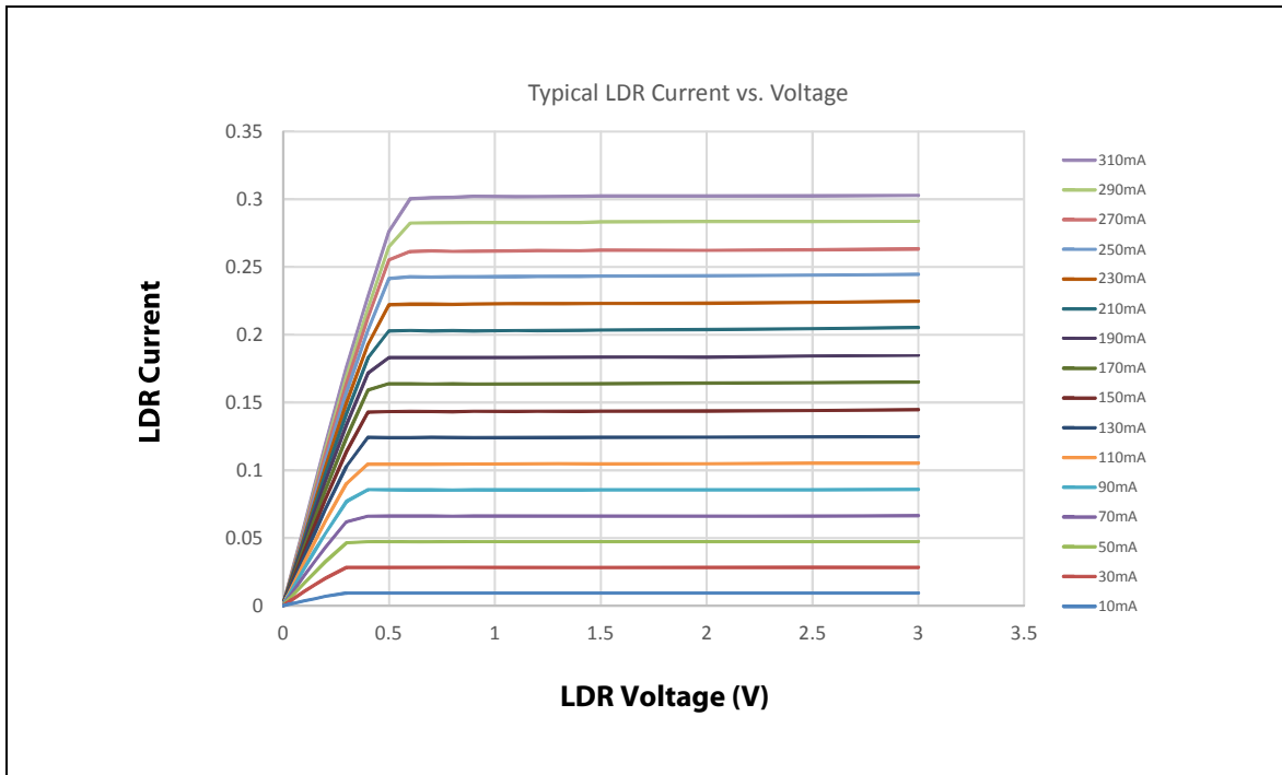
Figure 18: Typical LDR Current vs. Voltage
