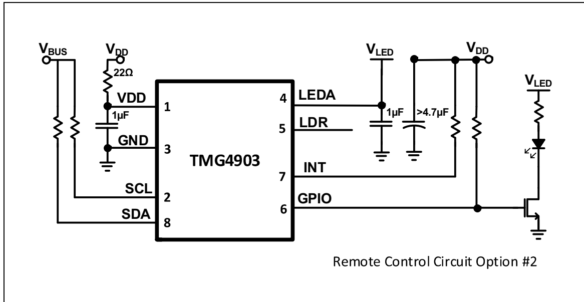
Figure 97: External IR LED Using the GPIO Pin
