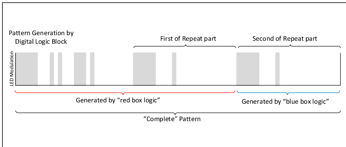
Figure 93: Pattern Generation by Logical Block
