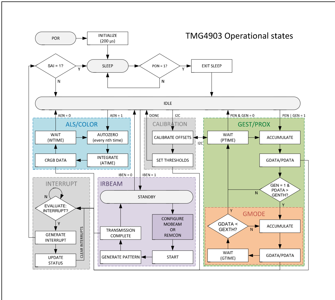
Figure 26: Detailed State Diagram
