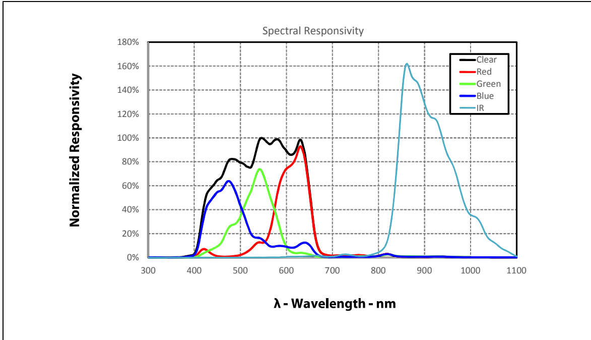
Figure 16: Spectral Responsivity
