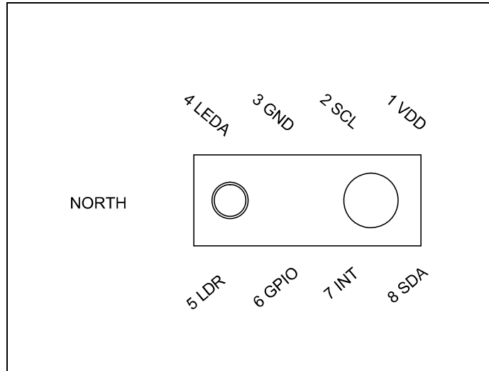
Figure 3: Pin Diagram
