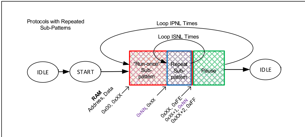
Figure 91: Number of Repeated Sub-Pattern Loops
