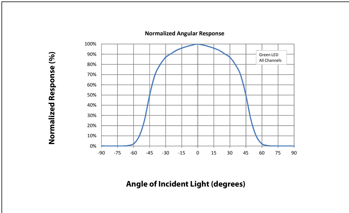
Figure 17: CRGB Responsivity vs. Angular Displacement
