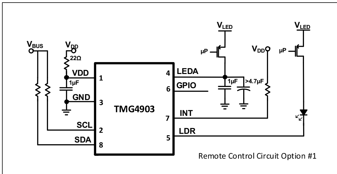
Figure 96: External IR LED Using the LDR Pin
