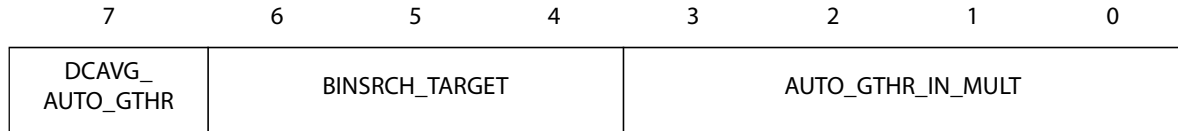
Figure 76: Calibration Configuration Register Two
