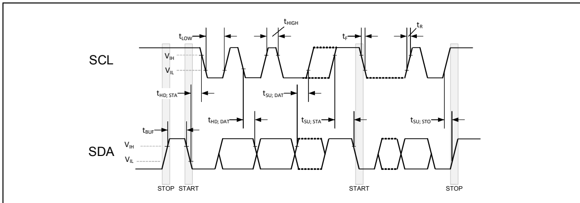
Figure 15: Timing Parameter Measurement Drawing
