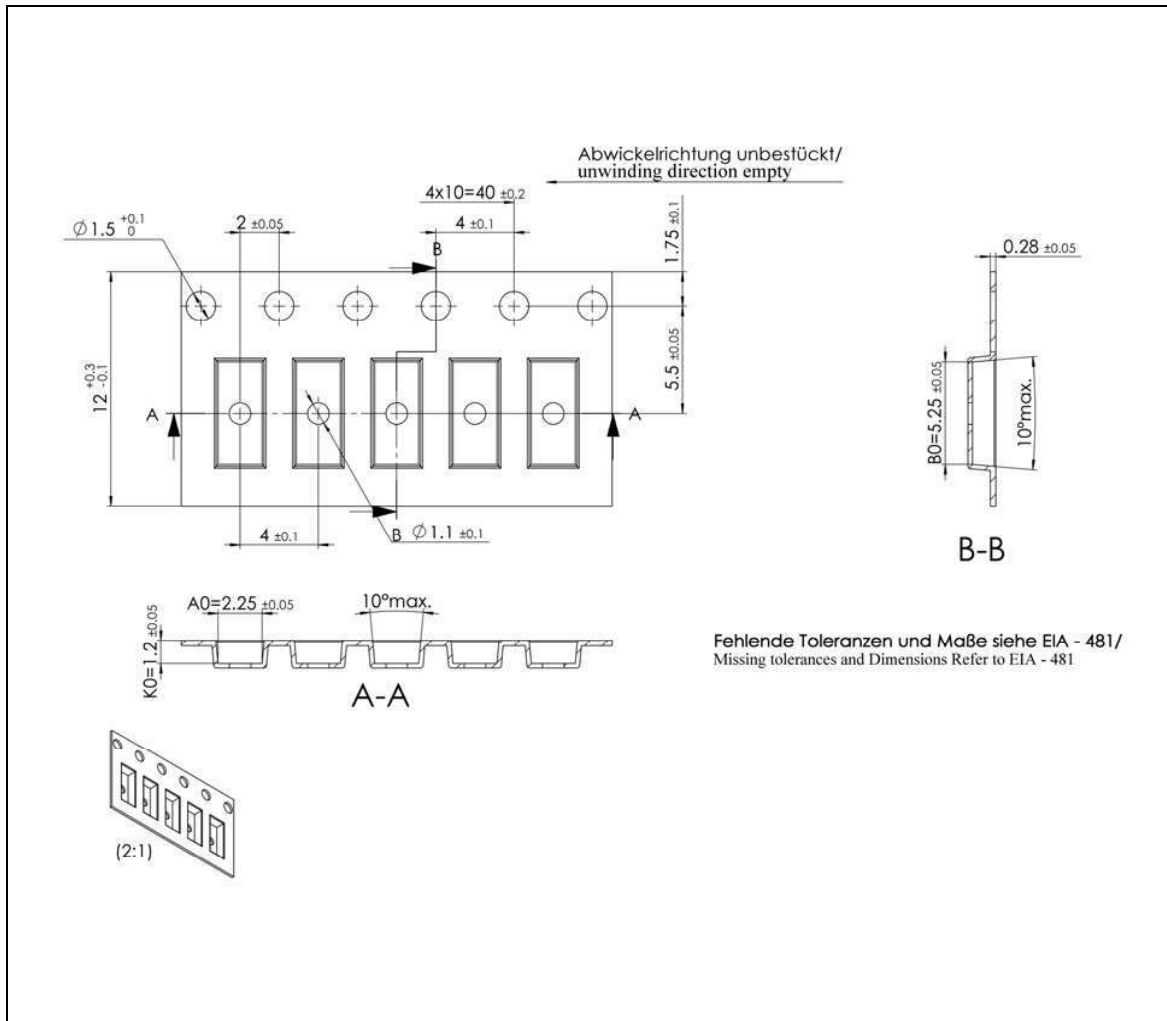
Figure 101: Tape and Reel Mechanical Drawing
