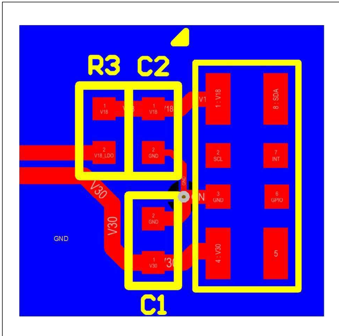
Figure 83: TMG4903 Recommended Circuit Layout
