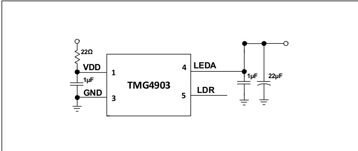
Figure 11: Proximity Test Circuit
