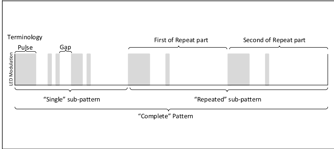
Terminology of Pattern RAM: Pulses/Gaps, and Single/Repeated/Complete Patterns are shown.
