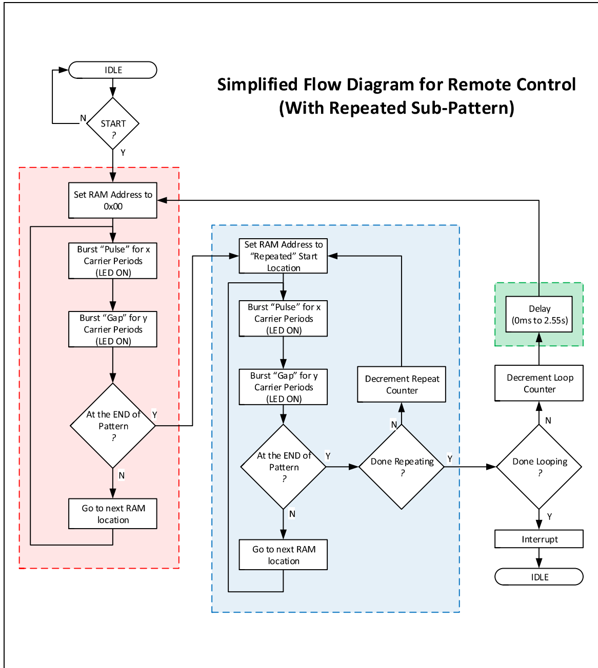
Figure 92: Simplified Flow Diagram
