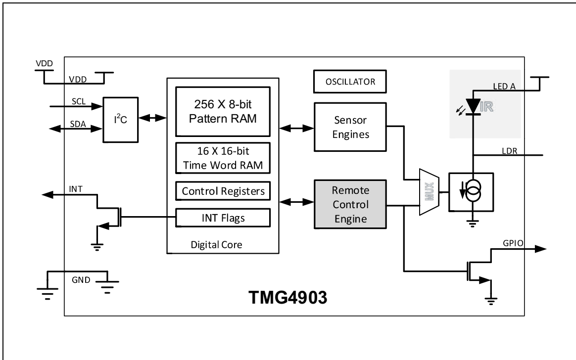
Block Diagram of RC Functionality: Resources associated with Remote Control.
