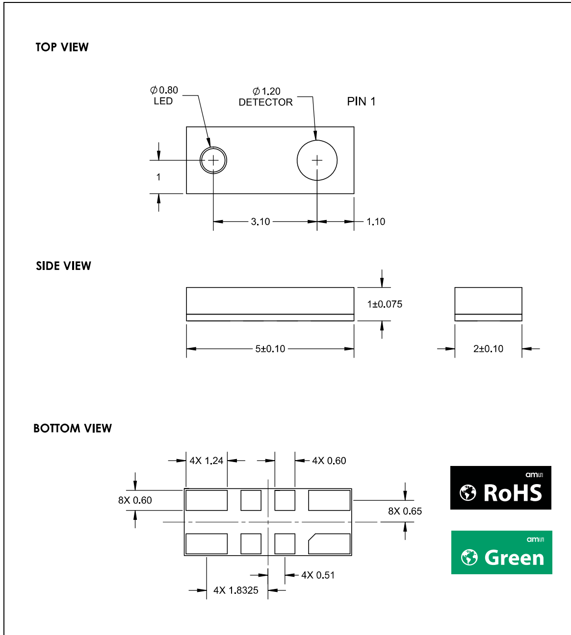
Figure 99: TMG4903 Module Dimensions
