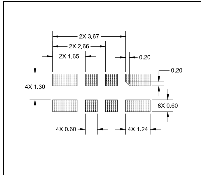
Figure 100: Recommended PCB Pad Layout
