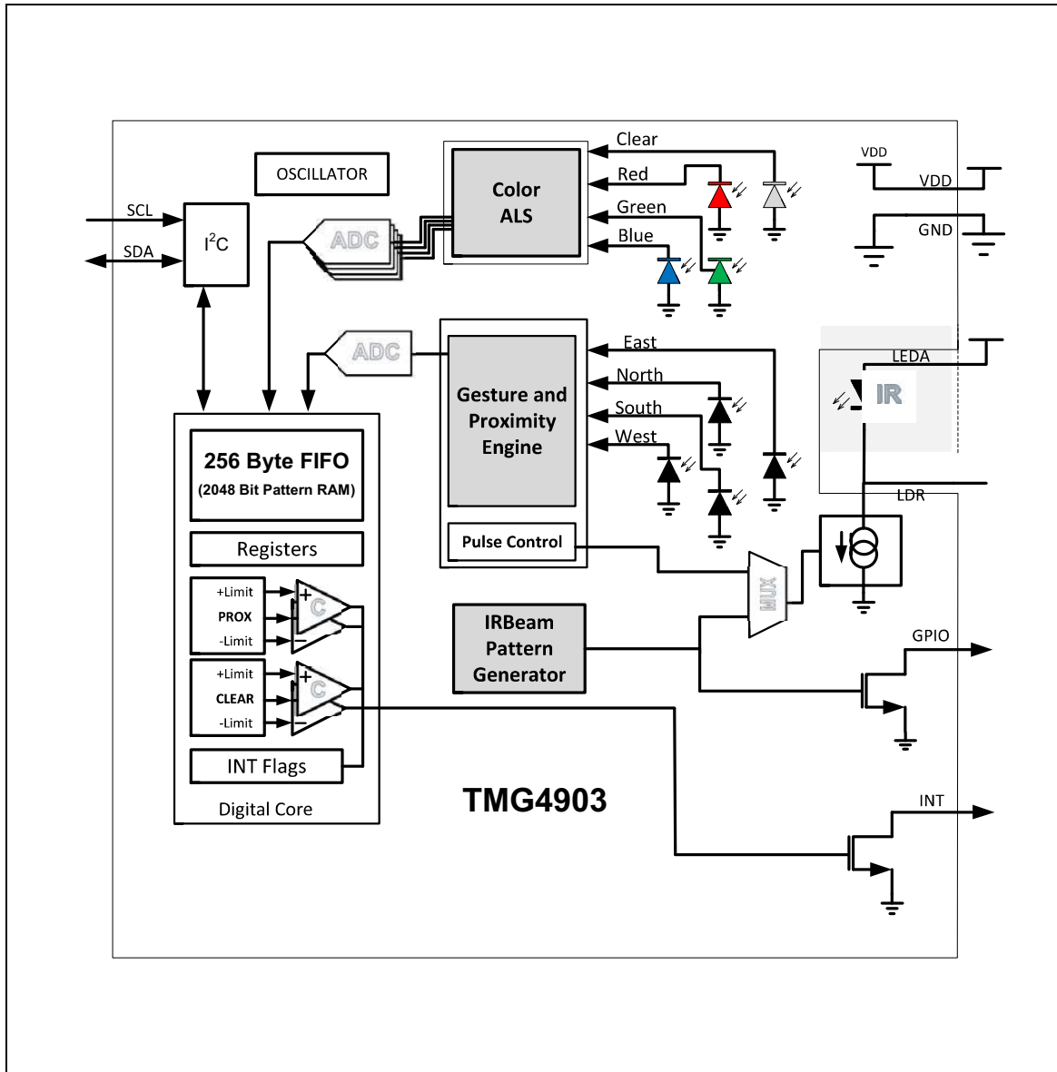
Figure 2: TMG4903 Block Diagram
