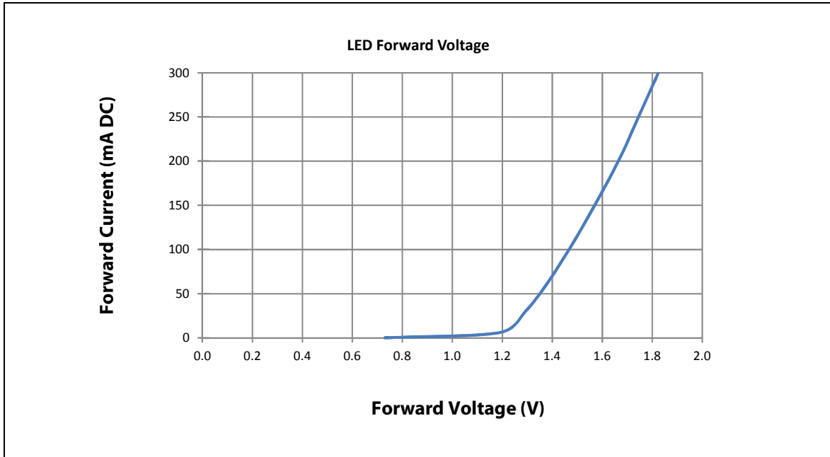
Figure 21: 950nm LED Forward Voltage vs. Current
