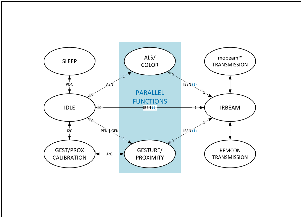
Figure 25: Simplified State Diagram
