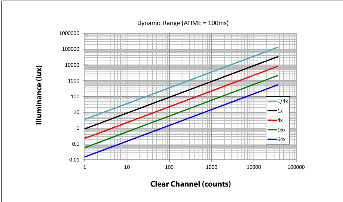
Figure 20: Illuminance (Lux) vs. Counts (Clear Channel)
