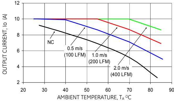
Figure 49. EQW010A0B-C/H, (12.0V, 10A).
