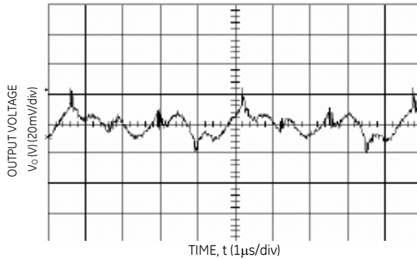
Figure 8. Typical output ripple and noise ( V_{IN} = V_{IN,NOM} , I_o = I_{o,max} ).
