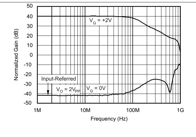
Figure 67. Fully-Attenuated Response
