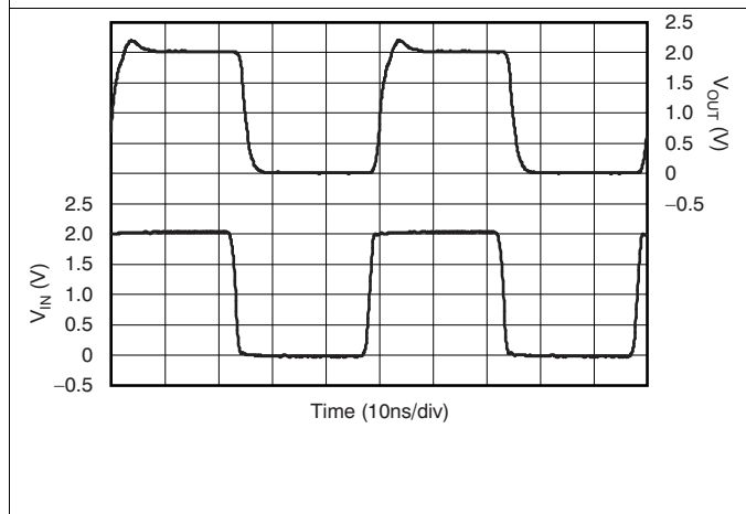
Figure 66. Gain Control Pulse Response
