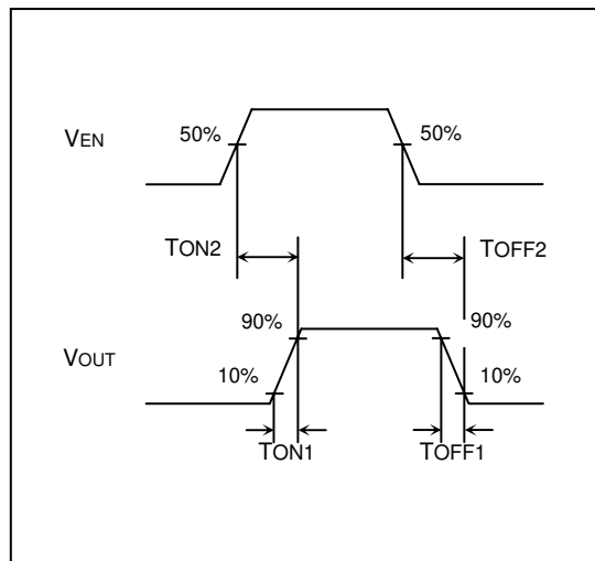
Figure 5. Output rise/fall time
