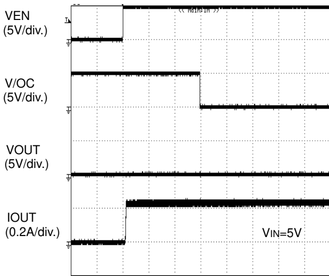
TIME (5ms/div.) Figure 36. Over-current response enable to shortcircuit
