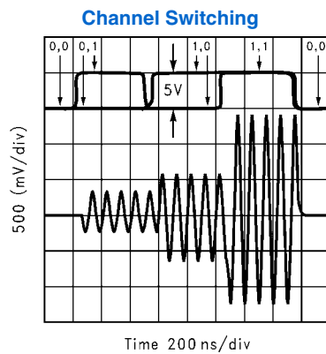
FIGURE 7. PGA Output
