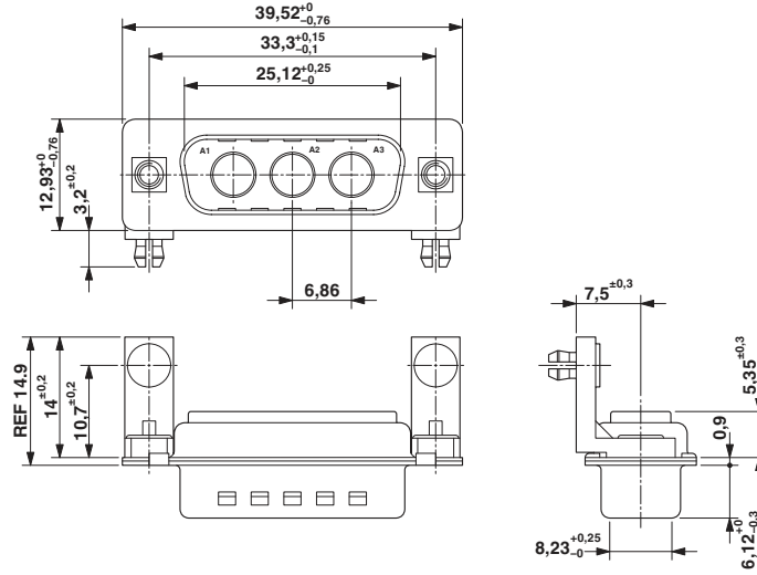
Dimensioned drawing
