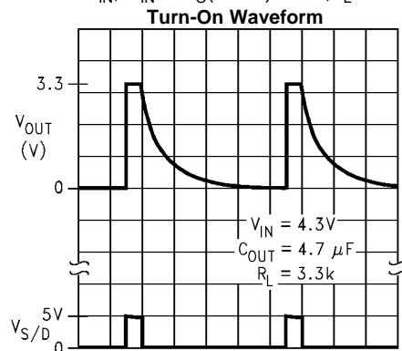
20 \text{ms}/\text{Div} Figure 18.
