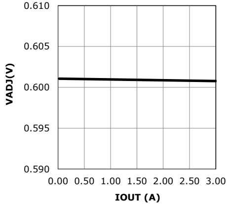
Fig. 4: VADJ versus IOU, 1.5VIN, 1VOUT
