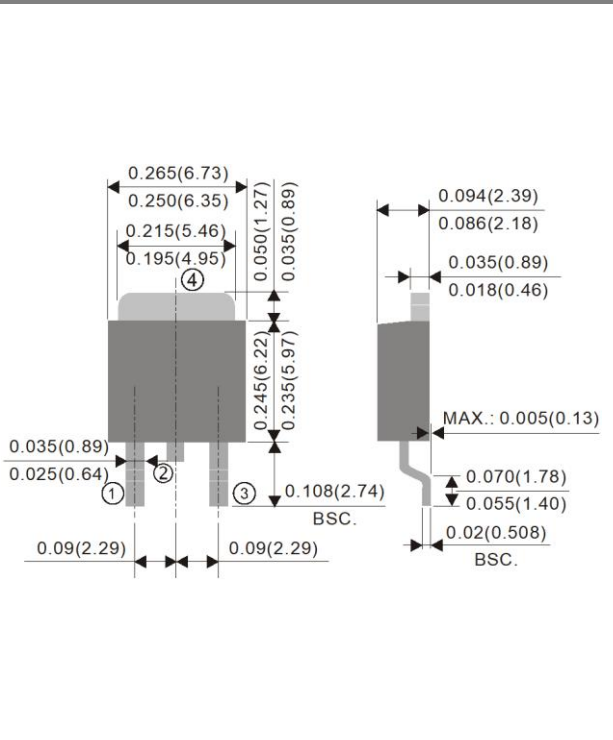
TO-252AA Dimension
