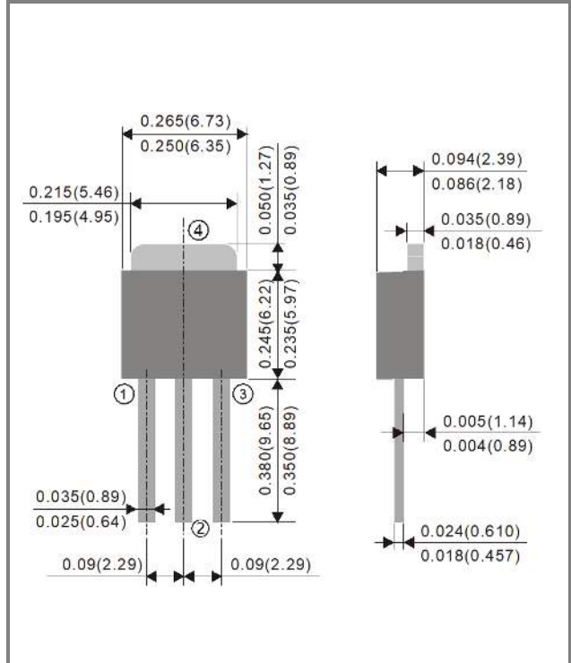
TO-251AA Dimension
