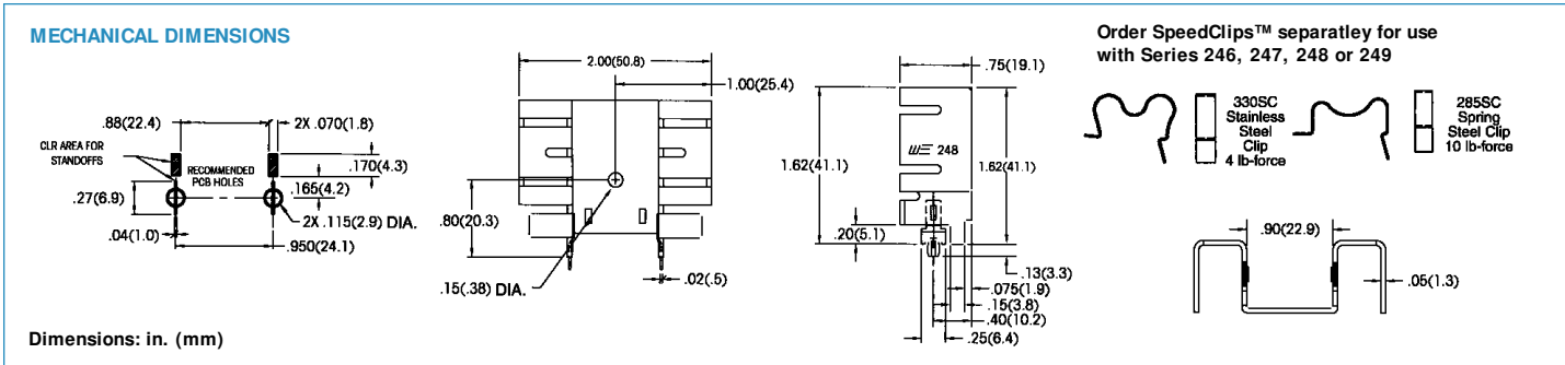
249 SERIES Medium Height, Deep Profile Wavesolderable Folded Fin Heat Sinks
