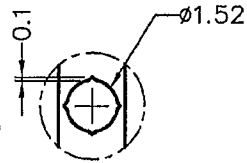
DETAIL SCALE 5:1
