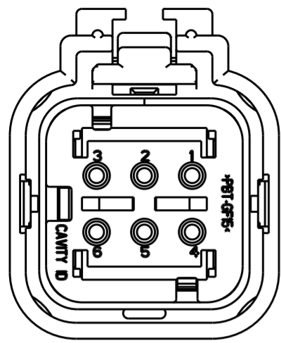
2098237-2 PURPLE TPA KEY B SCALE: 2:1
