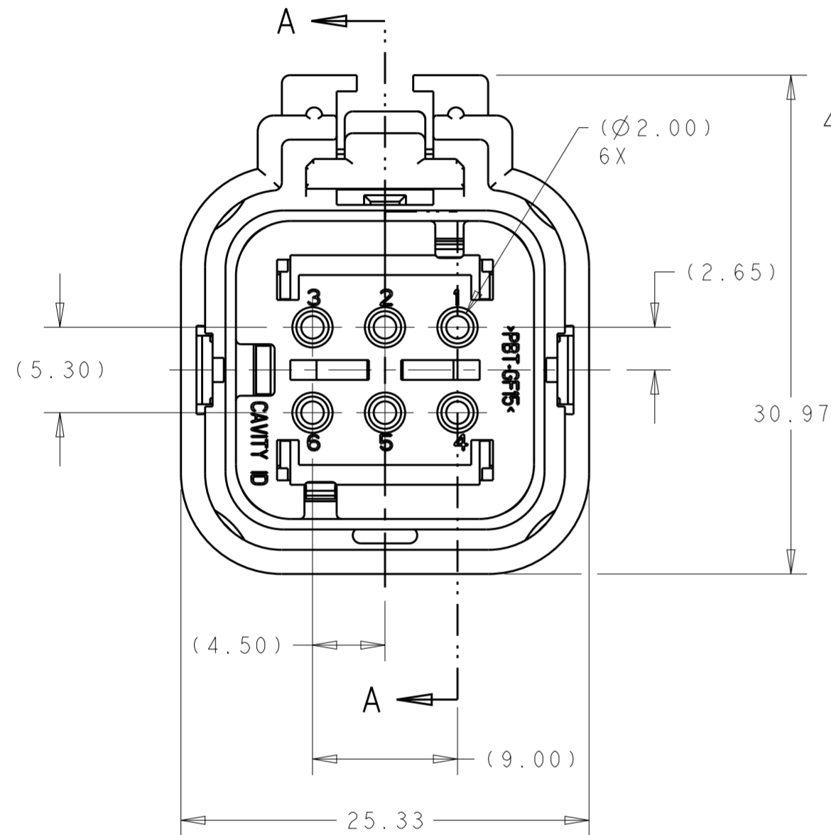
2098237-1 SHOWN ORANGE TPA KEY A
