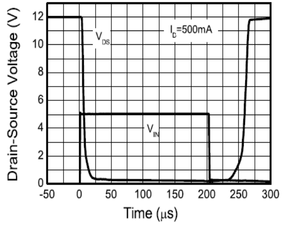
Switching Speed
