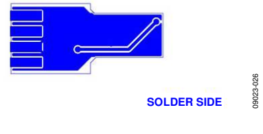
Figure 26. ADT7420FBZ Solder Side (Layer 2)
