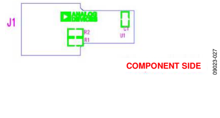
Figure 27. ADT7420FBZ Silkscreen
