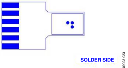
Figure 23. ADT7320FBZ Solder Side (Layer 2)
