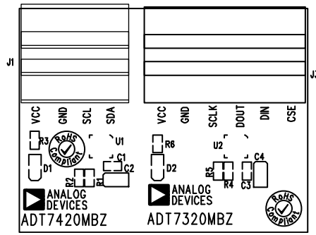
Figure 21. ADT7x20 Evaluation Board External Board Silkscreen
