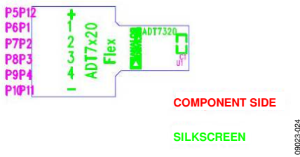
Figure 24. ADT7320FBZ Silkscreen
