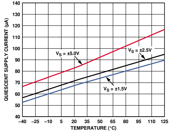
Figure 44. Sleep Mode Quiescent Supply Current vs. Temperature
