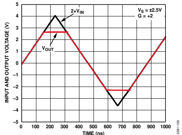
Figure 33. Output Overdrive Recovery Time
