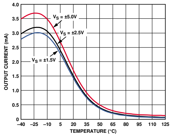
Figure 45. Sleep Mode Output Current vs. Temperature
