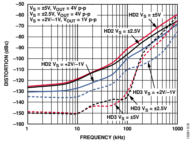
Figure 16. Distortion vs. Frequency, G = +2
