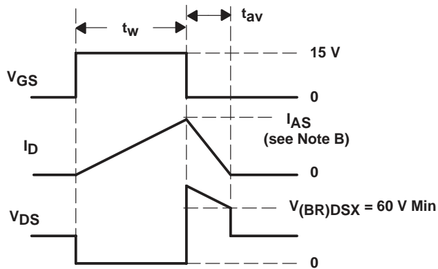
VOLTAGE AND CURRENT WAVEFORMS
