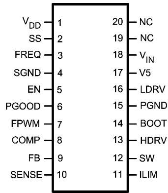
Top View 20-Lead TSSOP (MTC)
