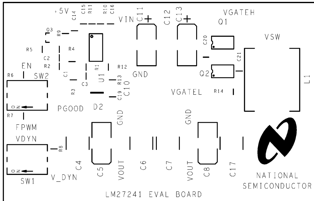
FIGURE 18. Top Overlay
