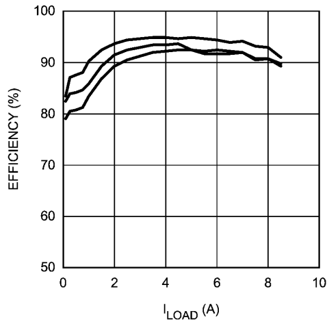
Efficiency for 2.5V Output
