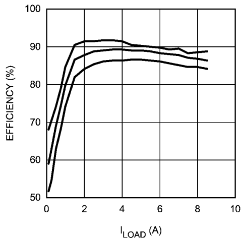
Efficiency for 1.05V Output
