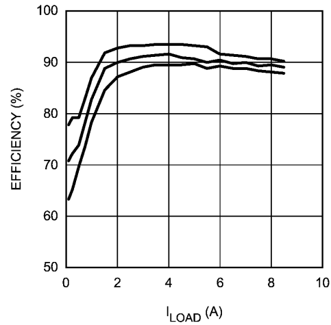
Efficiency for 1.5V Output
