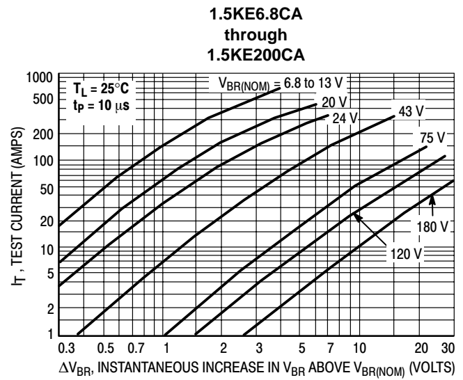
Figure 6. Dynamic Impedance
