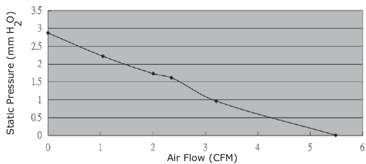
CFM-4010B-165-251
