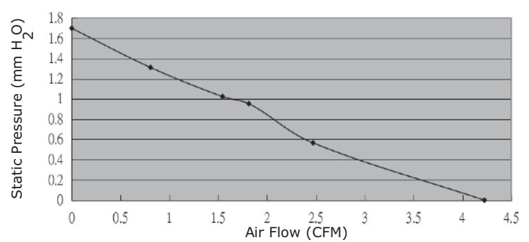
CFM-4010B-150-195
