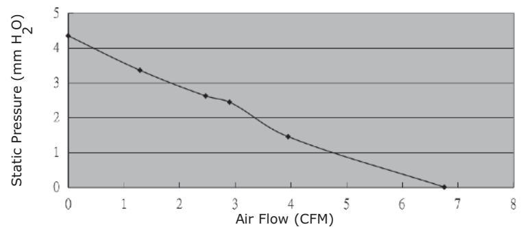
CFM-4010B-180-296
