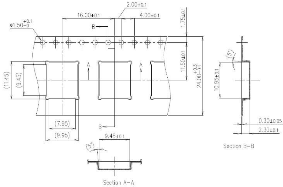
Figure 42. Tape Dimension
