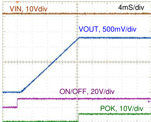
Figure 19. On/Off Enable wave form @+25°C (VIN=12V, VOUT=1.8V, IOU=4A)
