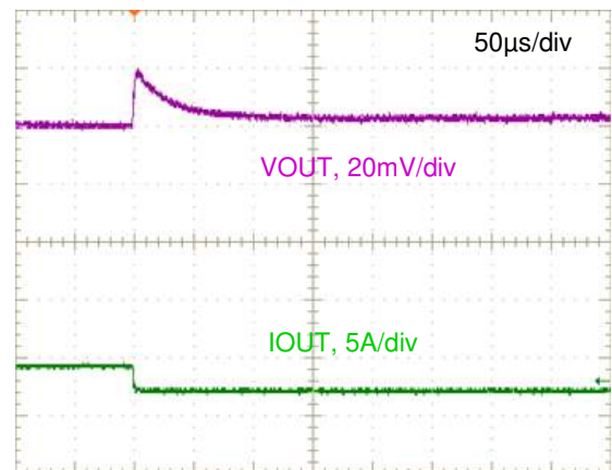
Figure 22. Step Load Transient Response (VIN=12V, VOUT=1.8V, COU=200µF, IOU=4 to 2A, 1.0A/µs)
