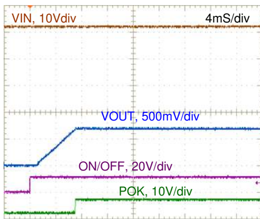
Figure 31. On/Off Enable wave form @+25°C (VIN=12V, VOUT=0.7V, IOUT=4A)
