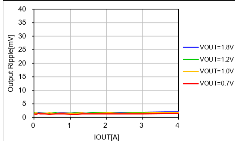
Figure 6. Output Ripple vs. Load Current and Output Voltage (COU=200μF, ScopeBW=20MHz)
