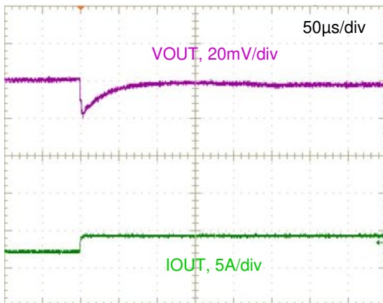
Figure 21. Step Load Transient Response (VIN=12V, VOUT=1.8V, COU=200µF, IOU=2 to 4A, 1.0A/µs)
