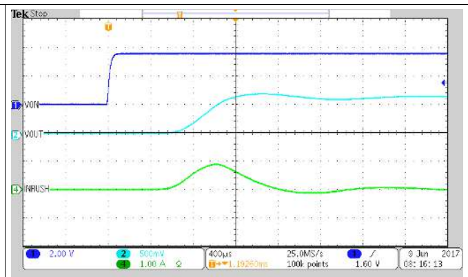
Figure 22. TPS22970 Inrush Current at 0.65 V IN With C L = 800 µF
