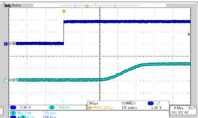
Figure 10. Turn-ON Response at 3.6 V_{IN}
