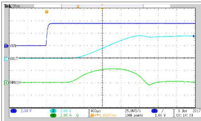
Figure 21. TPS22970 Inrush Current at 3.6 V IN With C L = 800 µF
