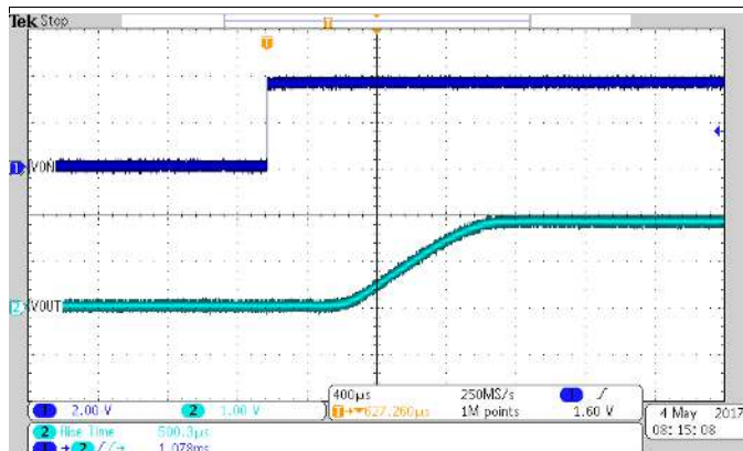
Figure 11. Turn-ON Response at 1.8 V_{IN}
