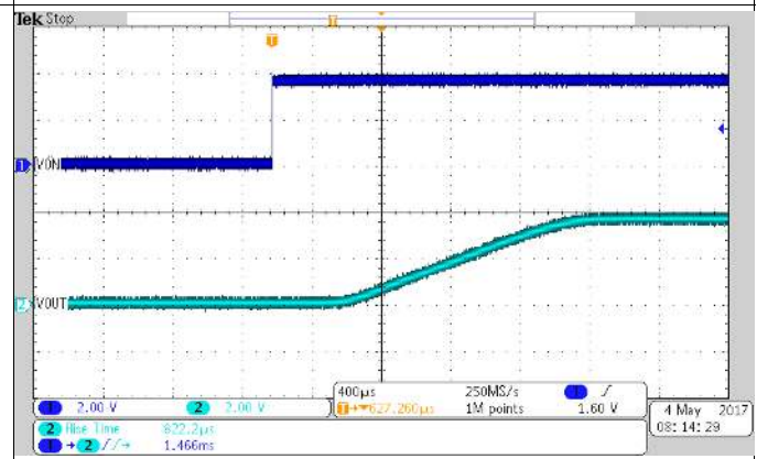
Figure 10. Turn-ON Response at 3.6 V_{IN}
